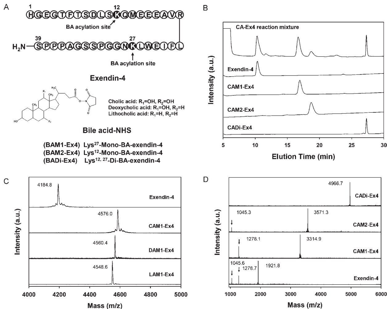
Figure 1. Preparation, purification, and structural characterizations of BA-Ex4s. (A) Chemical structures of BA-NHSs, the amino acid sequence of exendin-4, and of its BA acylated derivatives. (B) Reversed phase HPLC chromatograms of a CA acylation reaction mixture (CA/exendin-4 feed ratio of 1/1) and of purified CA-Ex4s. (C) Total mass spectra of exendin-4 and BAM1-Ex4s, obtained by MALDI-TOF MS. (D) Mass spectra of CA-Ex4s after Lys-C enzymatic digestion.
